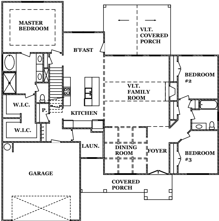
FIRST FLOOR
