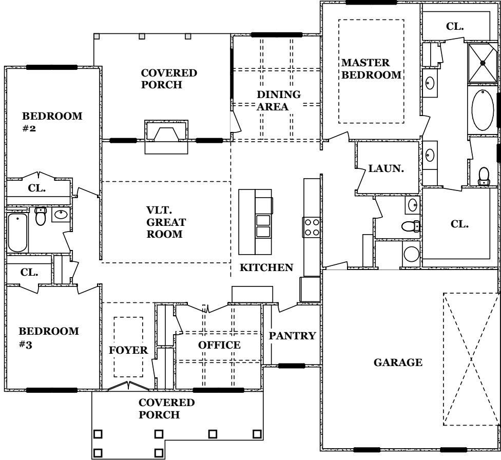
FLOOR PLAN
