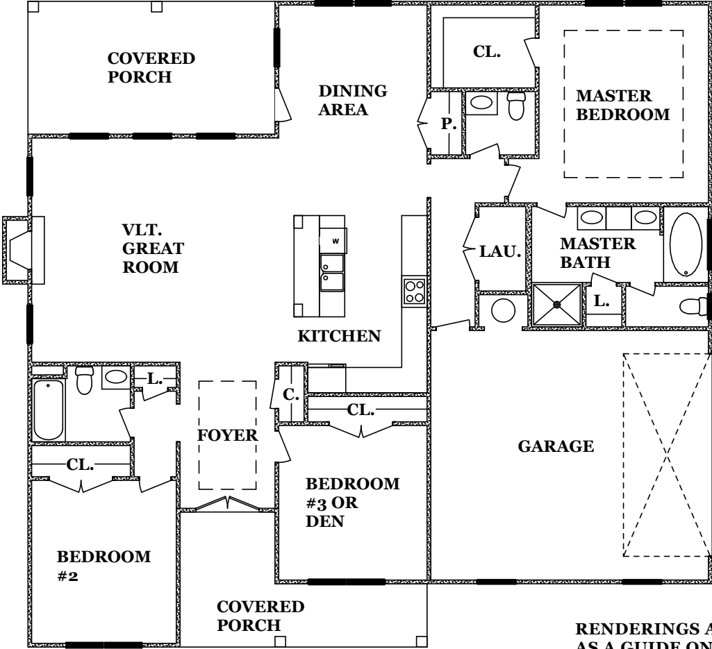
FLOOR PLAN
