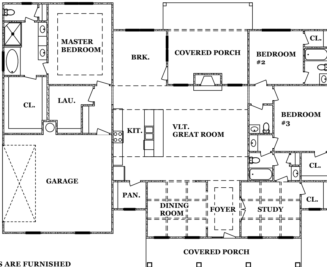
FLOOR PLAN
