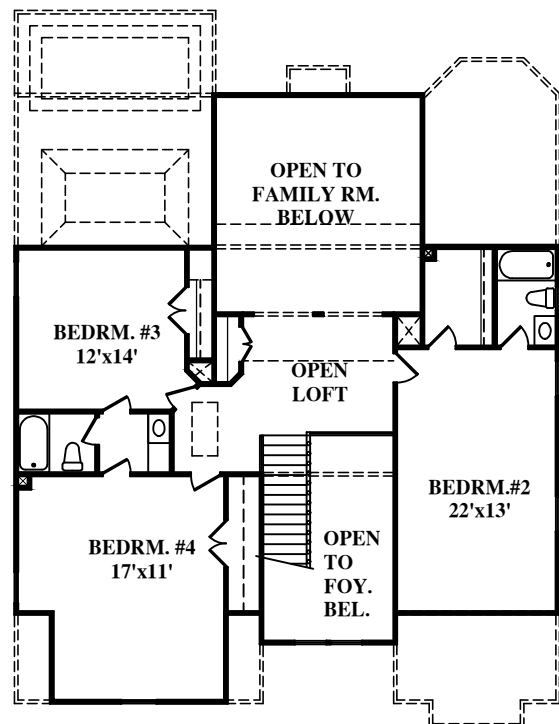
SECOND FLOOR 1,200 HSF
