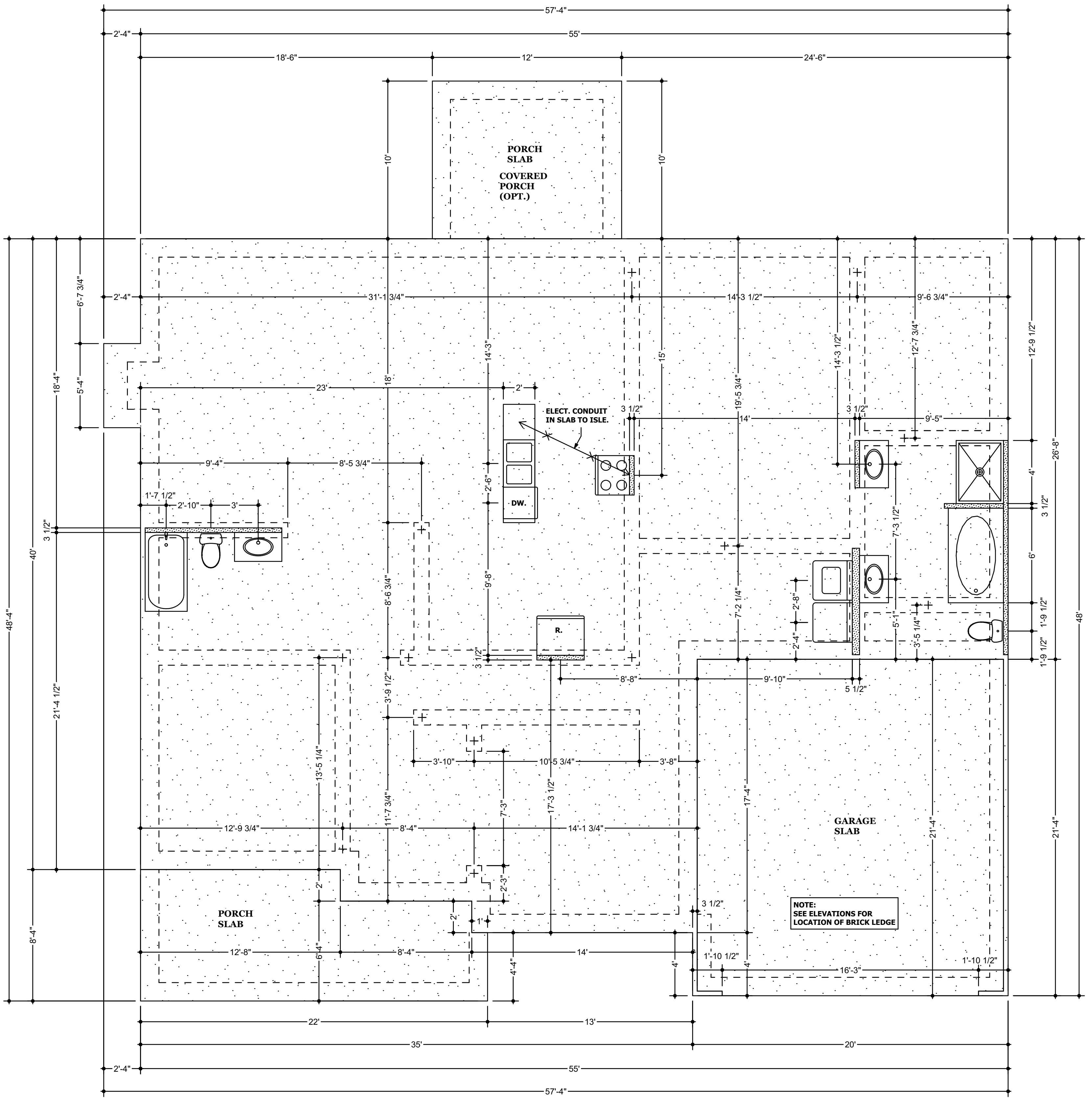
SLAB VIEW 1/4" = 1'-0"
