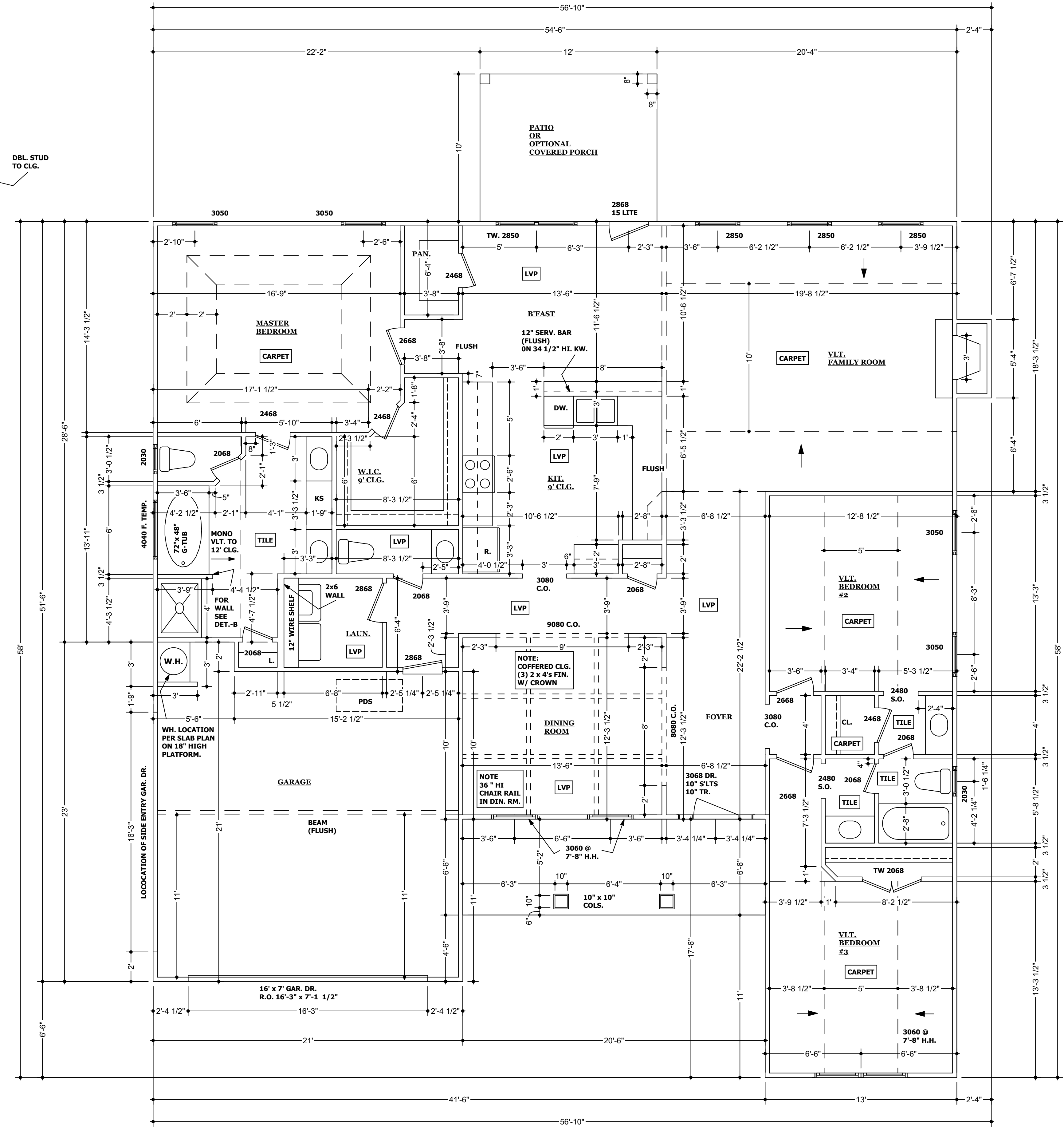
FLOOR PLAN 1/4" = 1'-0"
