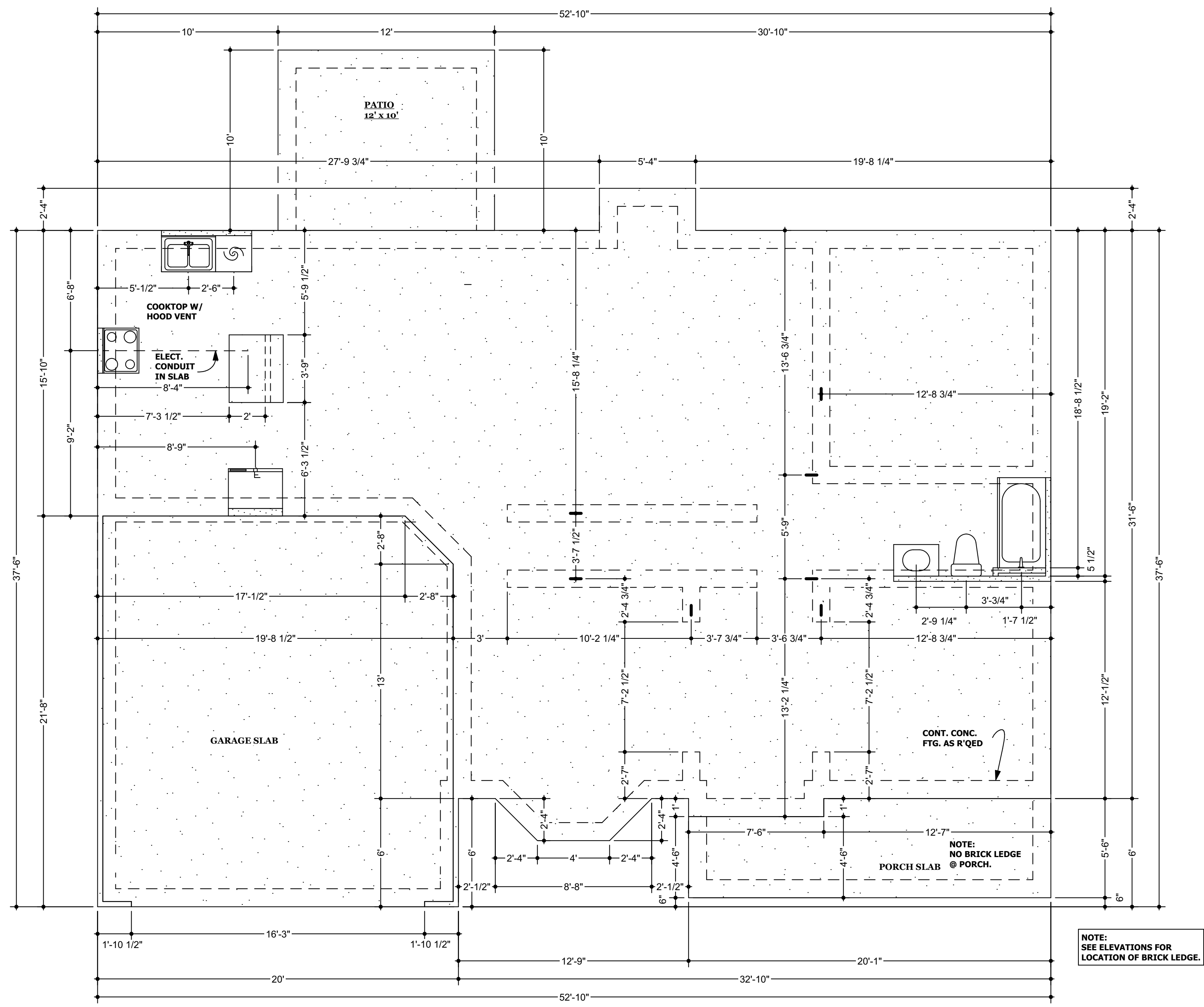
SLAB PLAN 1/4" = 1'-0"
