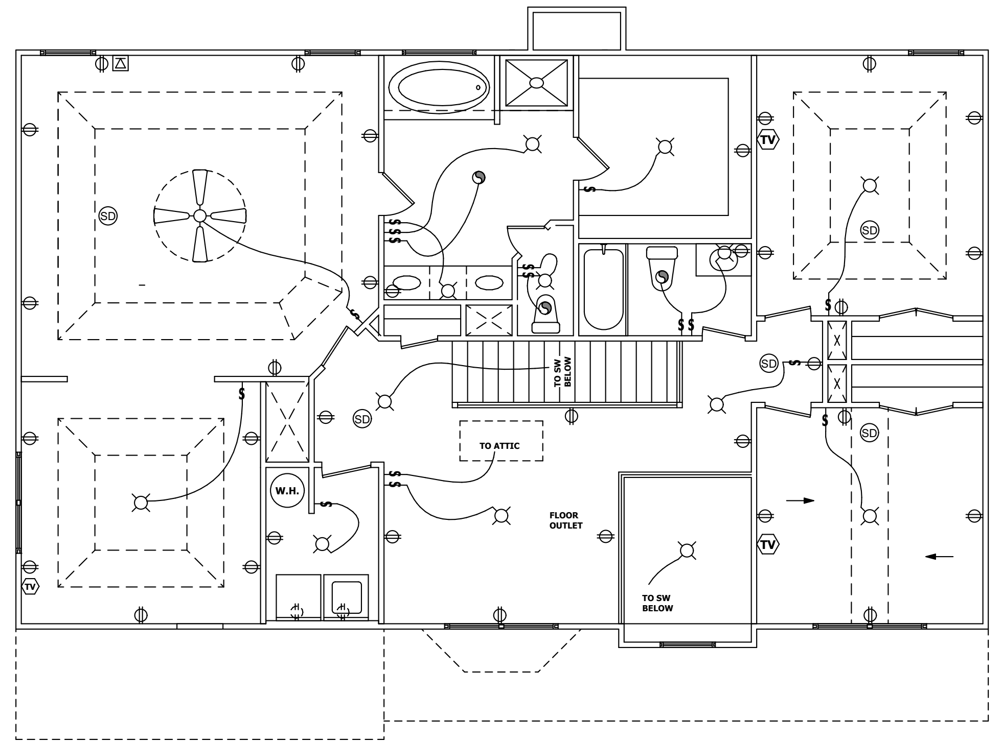
SECOND FLOOR ELECT. PLAN N.T.S.
