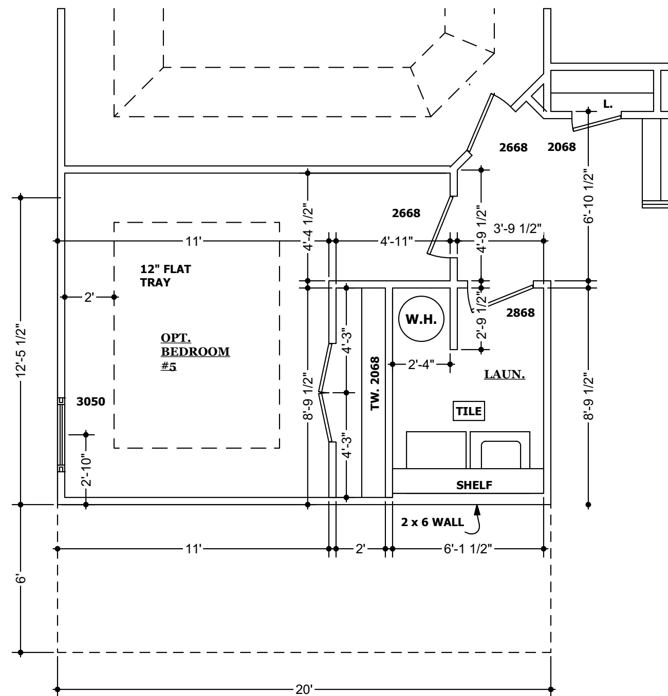
OPT. BR. # 5 1/4" = 1'-0"
