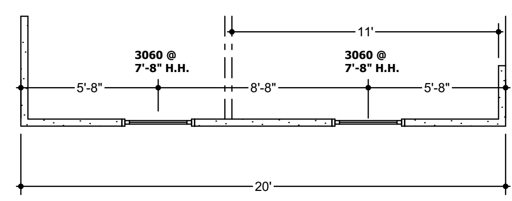
SIDE ENTRY GARAGE PLAN 1/4" = 1'-0"
