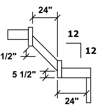
BR.# 2 & 4 TRAY DETAIL
