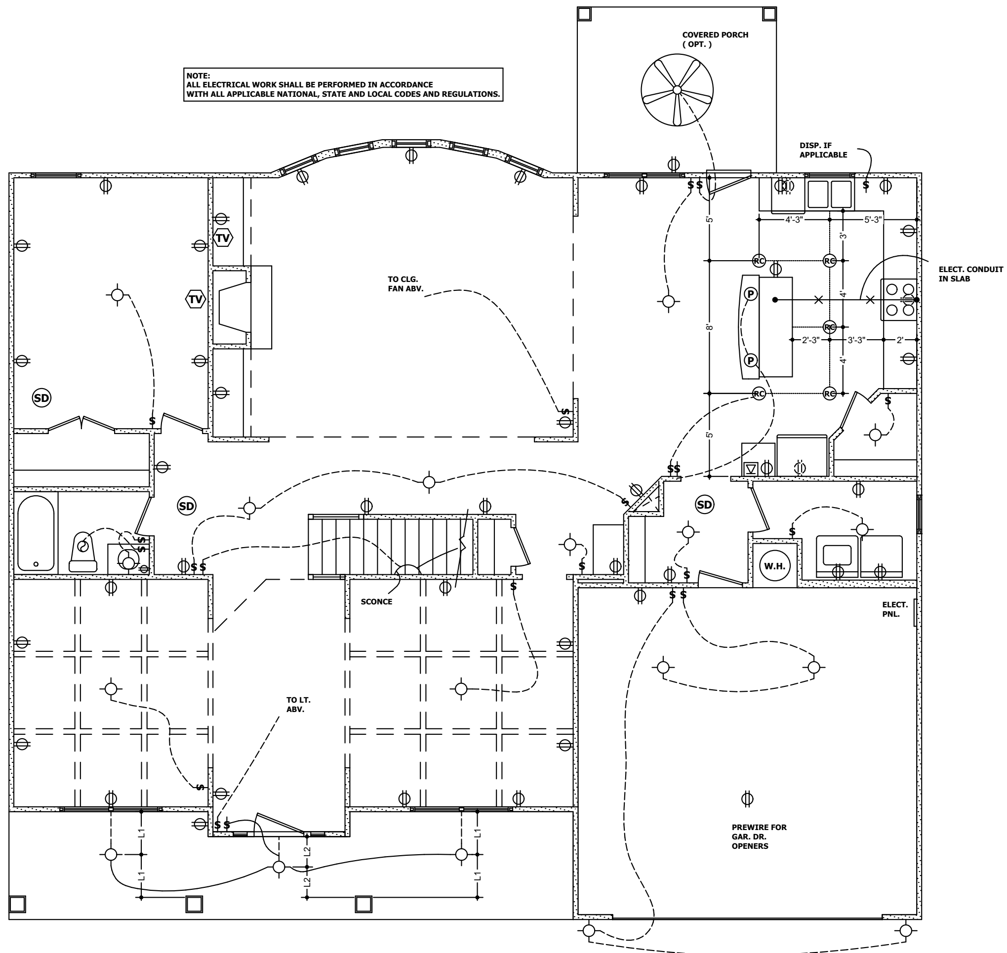
FIRST FLOOR ELECT. PLAN N.T.S.
