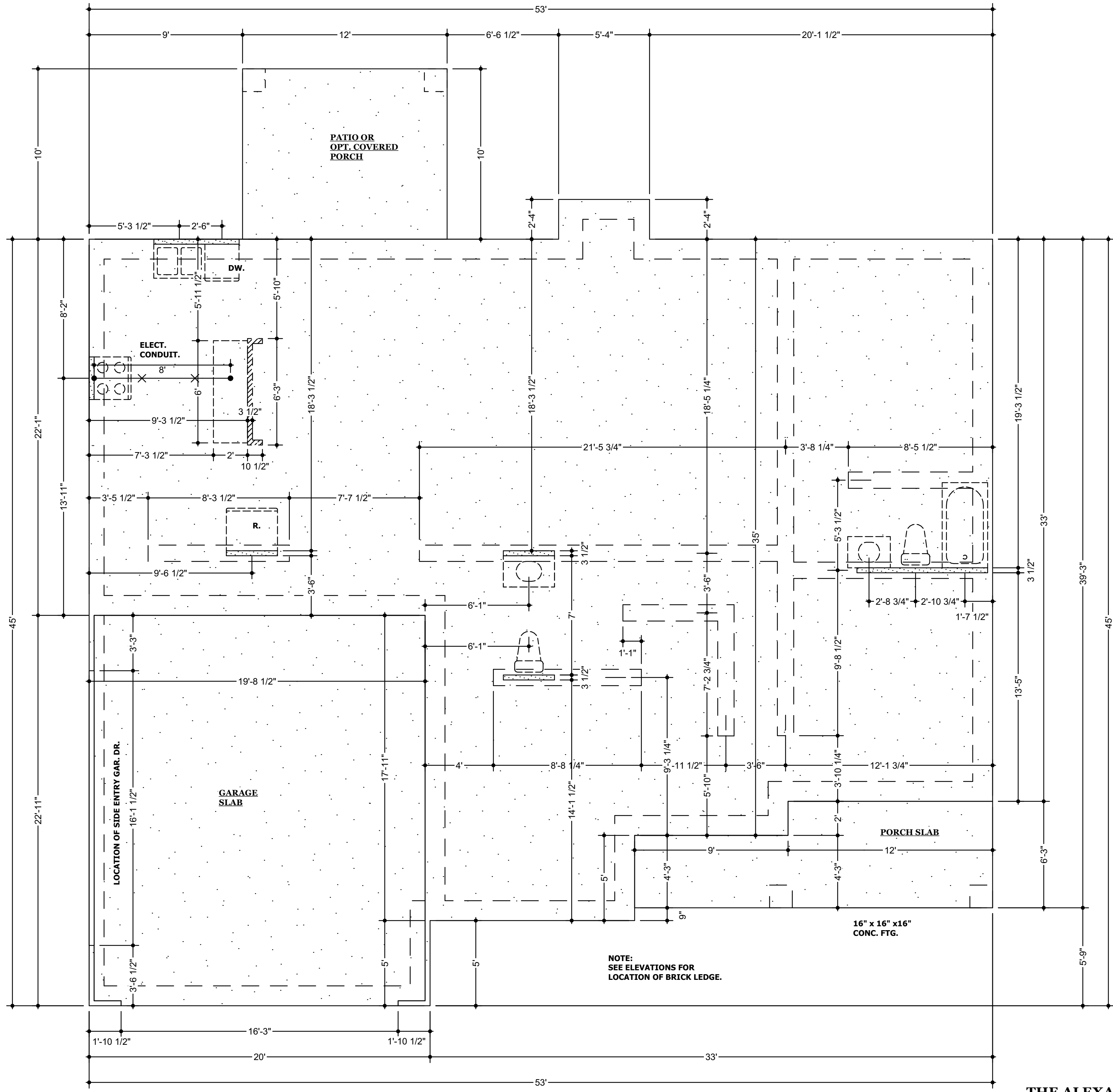
SLAB PLAN 1/4" = 1'-0"
