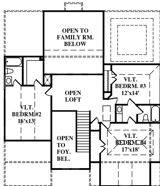
SECOND FLOOR 1,185 HSF
