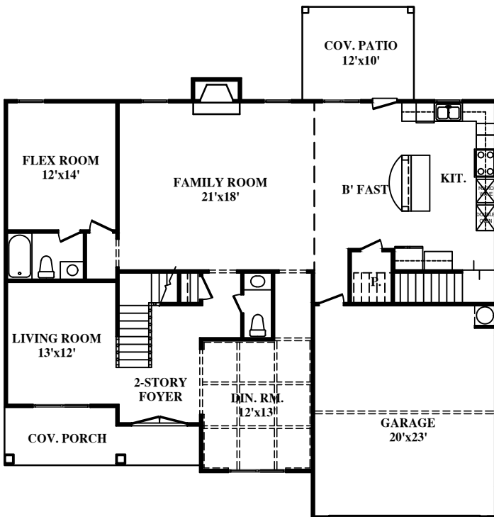
FIRST FLOOR 1,645 HSF
